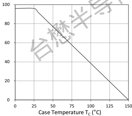
Figure 9. Power Dissipation
