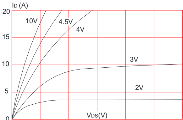
Figure 1: Output Characteristics
